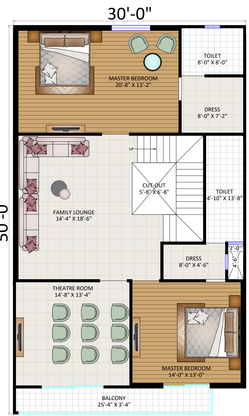
ROAD SECOND FLOOR PLAN
